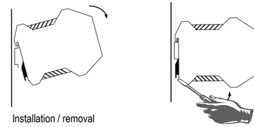
Installation / removal
