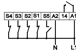
Fig. 1: Electrical Connection
