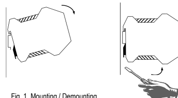
Fig. 1 Mounting / Demounting
