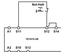
Fig. 4: Single-channel emergency stop circuit with earth fault monitoring. (category 1, up to PL c)
