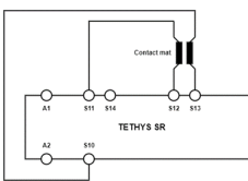
Fig. 7: Two-channel tactile sensor monitoring with short circuit and earth fault monitoring. (category 3, up to PL d)
