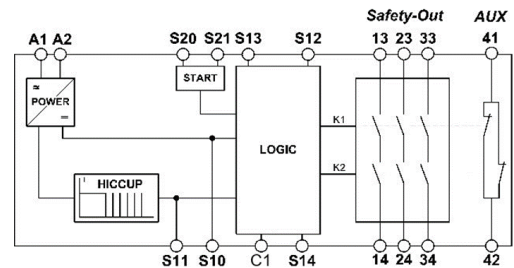
Fig. 1 Block diagram TETHYS IP65 SR
