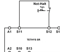
Fig. 5: Single-channel emergency stop circuit with earth fault monitoring. (category 1, up to PL c)
