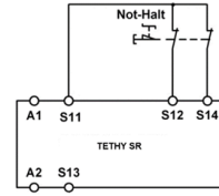
Fig. 3: Two-channel emergency stop circuit with earth fault monitoring. (category 3, up to PL d)
