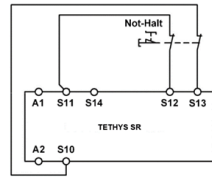
Fig. 2: Two-channel emergency stop circuit with short circuit and earth fault monitoring. (category 4, up to PL e)
