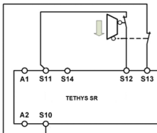
Fig. 6: Two-channel sliding guard monitoring with short circuit and earth fault monitoring. (category 4, up to PL e)
