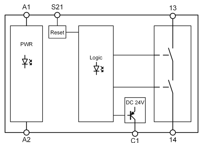
Fig. 2 Block diagram SD1E
