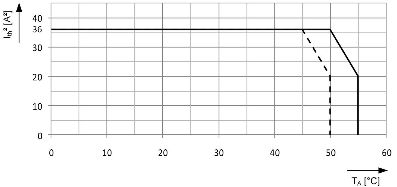
Fig. 8 Derating curve
