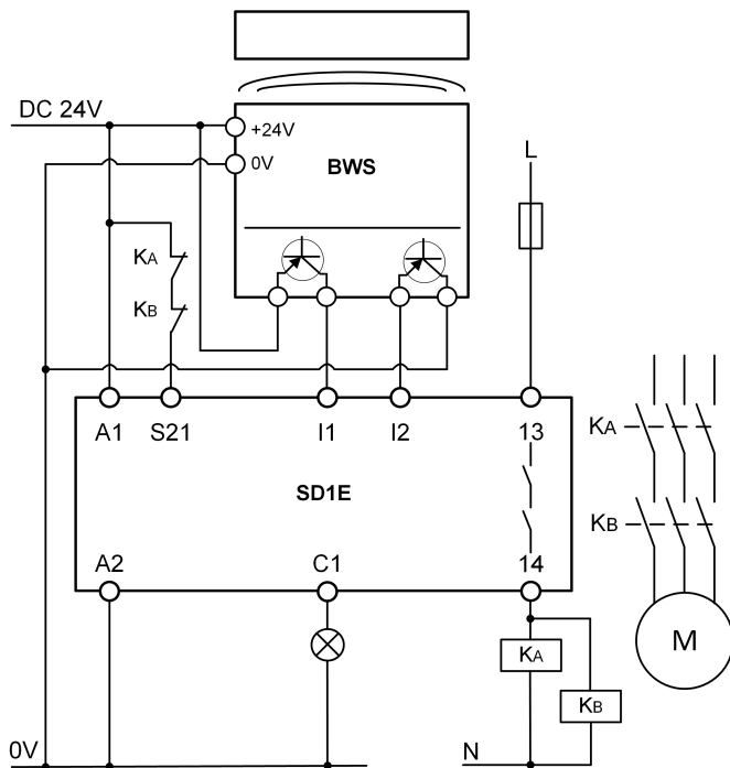
Fig. 5 Dual channel safety door monitoring with BWS
