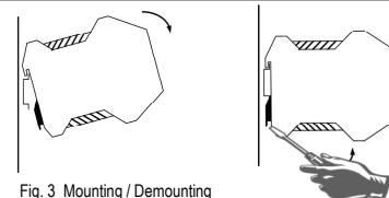
Fig. 3 Mounting / Demounting
