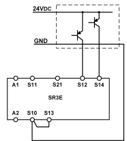
Fig. 9: Two channel emergency stop with pnp-outputs/OSSD-outputs with its own short circuit monitoring. (category 4, up to PL e / SIL 3) Prerequisite: Signal generator must meet requirements for PL e / SIL 3, too.
