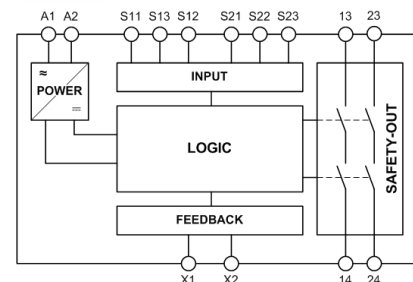
Fig. 1 Block diagram S2HC
