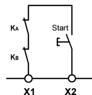
Fig. 5: Feedback loop
