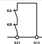
Fig. 12: Feedback loop for monitored manual start. The feedback loop monitors contactors or the expansion modules.
