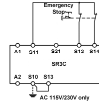
Fig. 4: Two-channel emergency stop circuit with short circuit and earth fault monitoring. (category 4, up to PL e)
