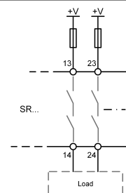
Fig. 14: Power supply A1 and A2. (Power supply according to techn. Data)
