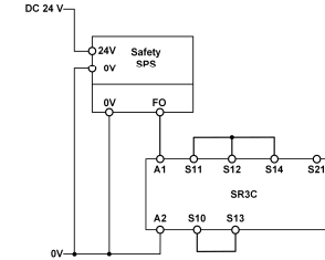
Fig. 9: Connecting to a safety PLC (category 4, up to PL e) Prerequisite: Fault exclusion for cross-circuit (e.g. according to EN ISO 13849-2; Table D4 - wiring in protected wiring space) and PLC also meets requirements for category 4, PL e.
