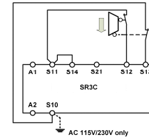
Fig. 6: Single-channel emergency stop circuit with earth fault monitoring. (category 1, up to PL c)
