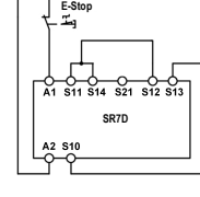
Fig. 9: Single channel emergency stop with ground fault monitoring. (Category 1, up to PL c / SIL 1)
