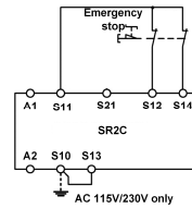
Fig. 4: Two-channel emergency stop circuit with short circuit and earth fault monitoring. (category 4, up to PL e, SIL 3)
