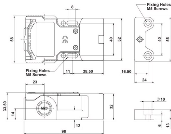
ZCode-KR switch (left) and actuator (right)
