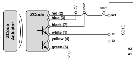
Figure 6: Single connection of a ZCode to one ZANDER MINOS SD1E (up to category 4, PL e)
