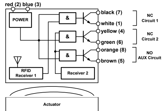
Fig. 2: Block diagram
