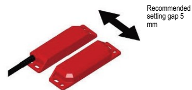
Fig. 3: Operating direction
