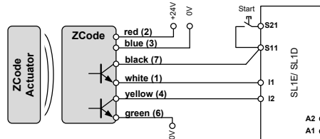
Figure 9 : Single connection of a ZCode to one ZANDER MINOS SL1D (up to category 3, PL d) / SL1E (up to category 4, PL e)
